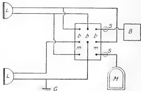
Diagram of Connection of Three-Pole Two-Throw Switch on Ford
